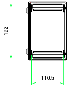
A-A (1:5.5)
