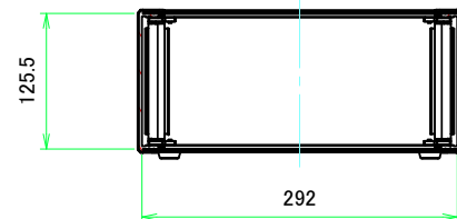
B-B (1:5.5)
